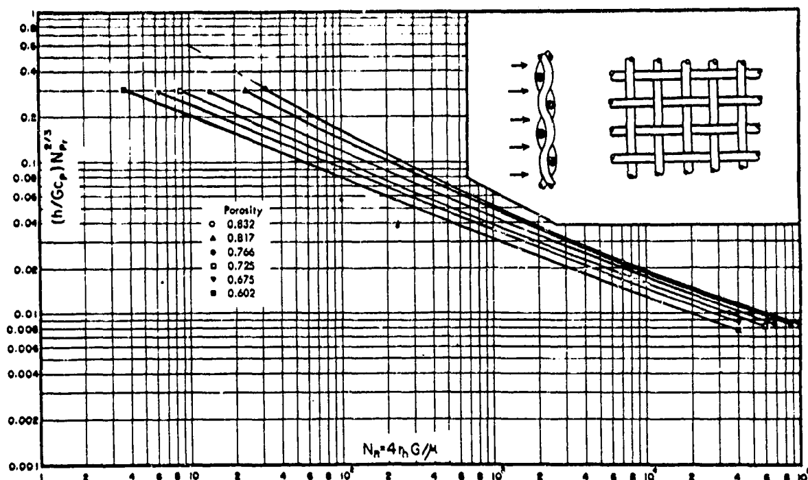
Figure A-6. Gas Flow Through an Infinite Randomly Stacked Woven-Screen Matrix, Heat Transfer Characteristics; a Correlation of Experimental Data from Wire Screens and Crossed Rods Simulating Wire Screens. Perfect Stacking, i.e., Screens Touching, is Assumed (64 1, p. 129).
