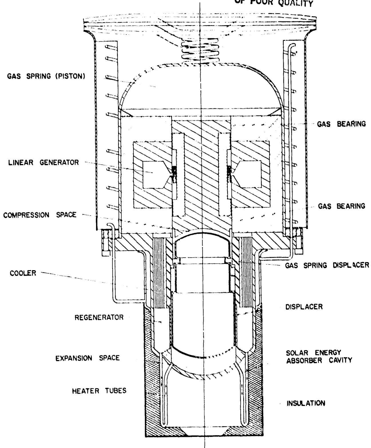
SUNPOWER 1 KILOWATT ENGINE SPIE
