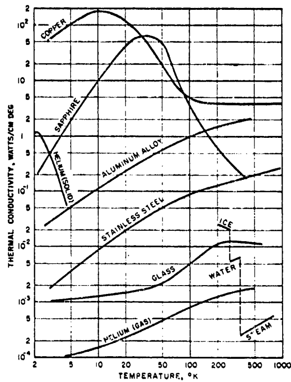
Figure A-3. Typical Curves Showing Temperature Dependence of Thermal Conductivity (From American Institute of Physics Handbook, 2nd Ed., pp. 4-79).
