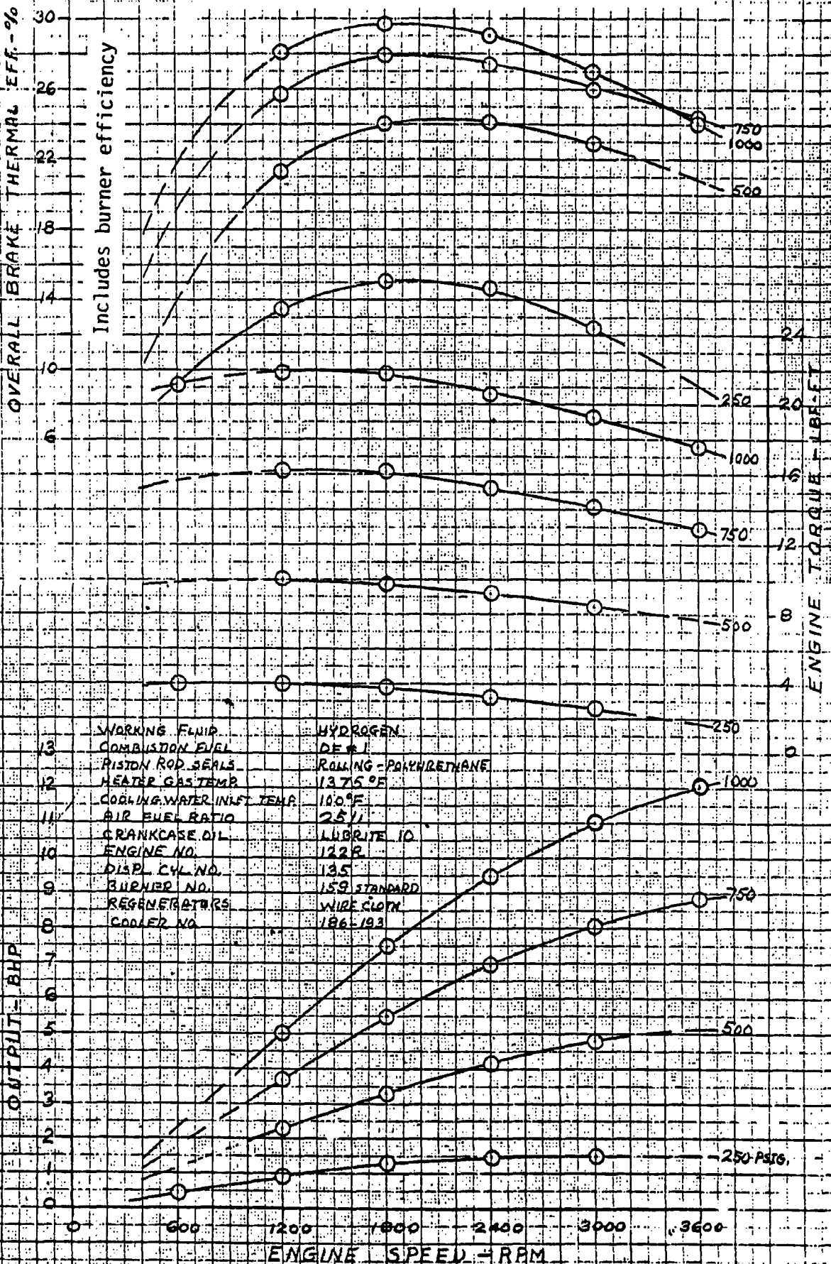
GPU-3 STIRLING THERMAL ENGINE PERFORMANCE - SPEED RUNS
