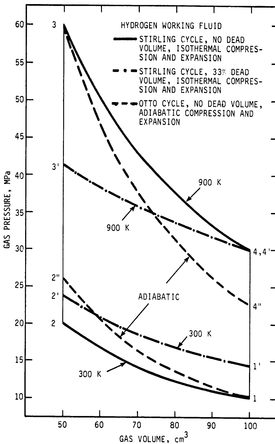
Figure 5-2. Theoretical Cycles.
