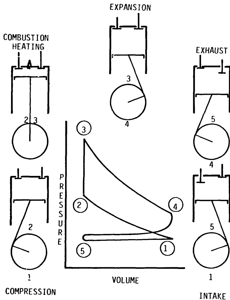
Figure 2-2. Example of Internal Combustion Engine.
