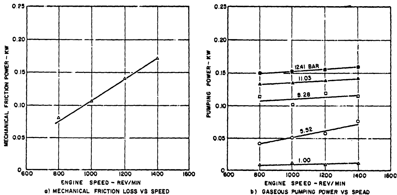
Figure 4-8. Possible Mechanical Friction and Gaseous Pumping Power of Stirling Air Engine as a Function of Engine Speed and Various Mean Operating Pressures.
