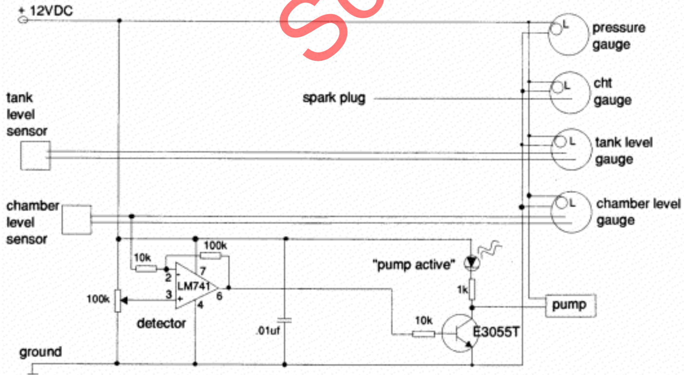
FIGURE 4 E-SCHEMATIC
