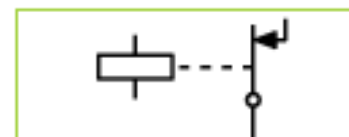
3 Normally closed (form B) contact graphic.
