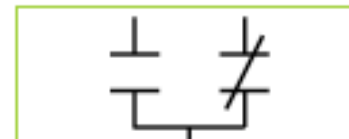
6 Changeover (form C) contact schematic.
